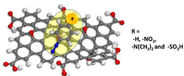
Figure 1. Representation of the used Graphene oxide 3D molecular model with substituted aryl diazonium cation.
