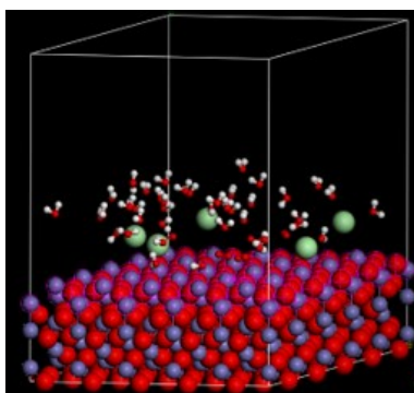
Figure 1. Slab model of Fe(001) surface together with chloride ions, oxygen molecules and water molecules.
