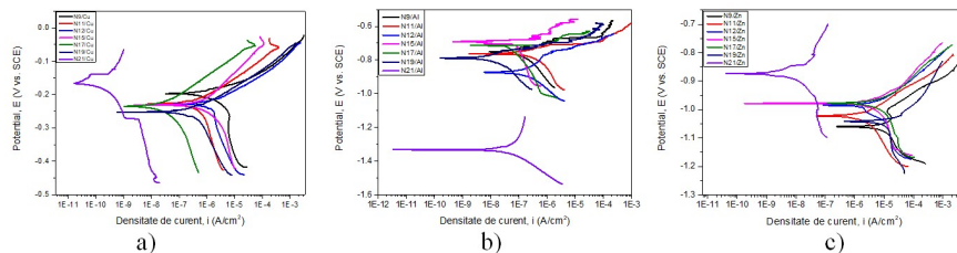
Figure 1. Tafel curves of metallic substrates a) Cu, b) Al, c) Zn, covered with different modified ZnO materials
