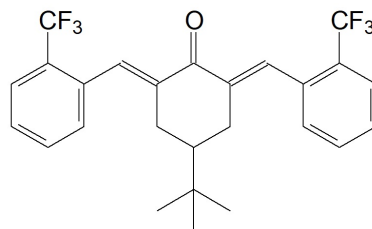
Figure 2. Structure of tert-Butyl-2,6-Bis[(2-trifluoromethyl)benzylidene]cyclohexanone
